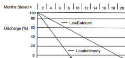
Figure 2 Self Discharge Rate Calcium vs. Antimony @ 77 °F
